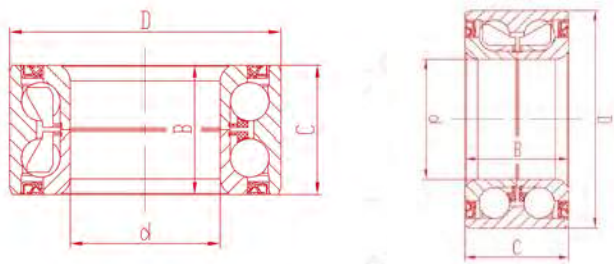
Basic Dimension Table G-AP to Dimension.....
